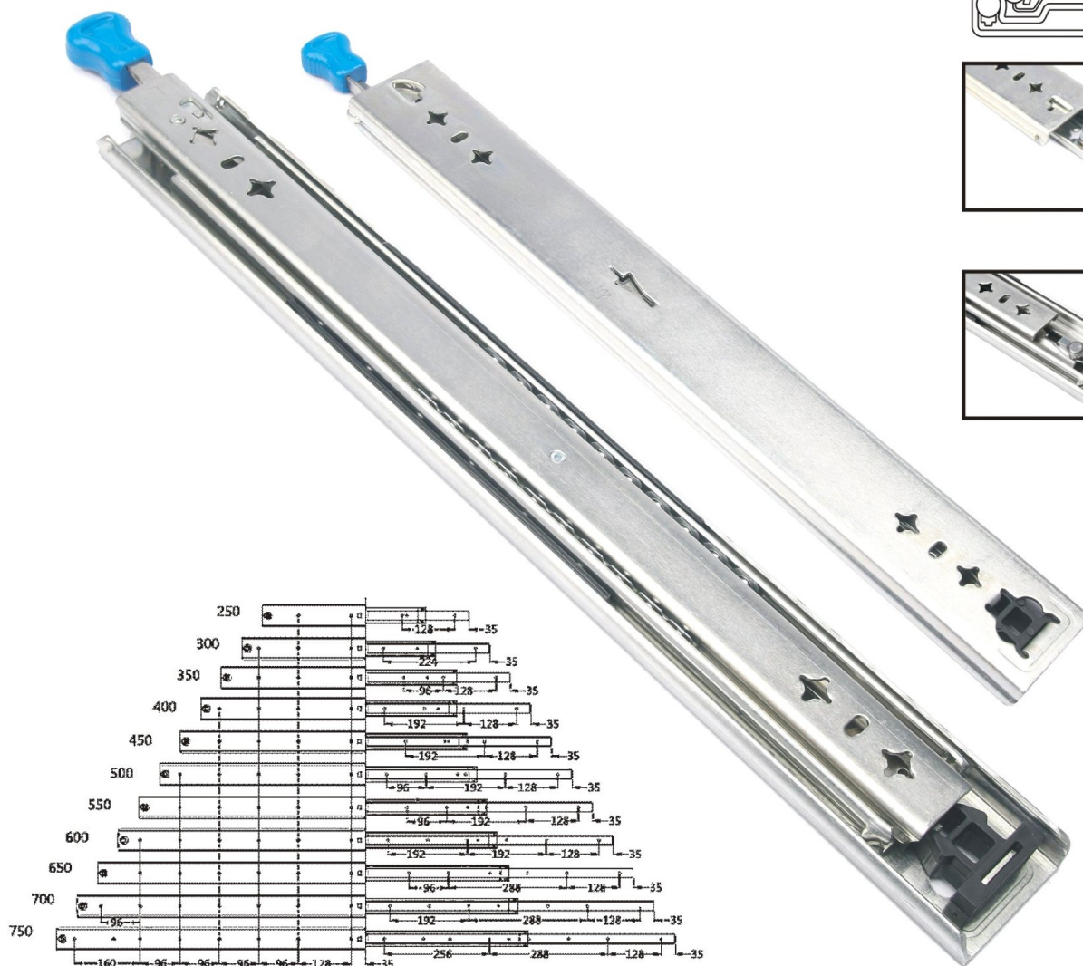
可拆卸扣 Removable clasp
