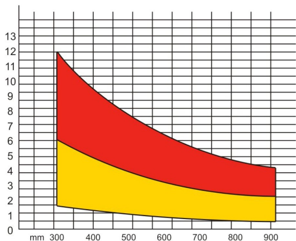
SUPPORT BEARINGCAPACITY · 支撑承载力说明图
