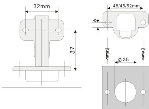
配自攻螺丝 with self-tapping screw
